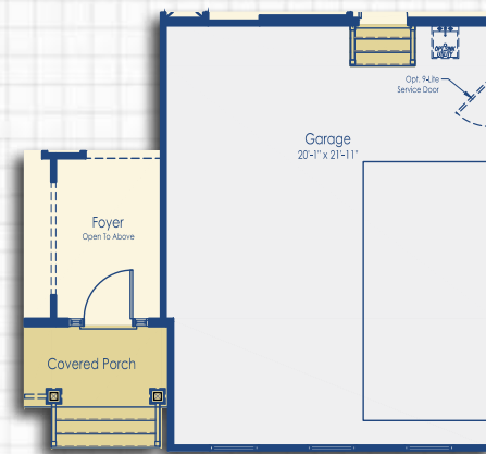
Optional Sideload Garage with 4ft Extension Southern Elevation
