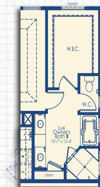
Optional Luxury Owner's Suite II
