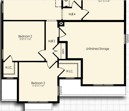
Included Elevation A Second Floor
