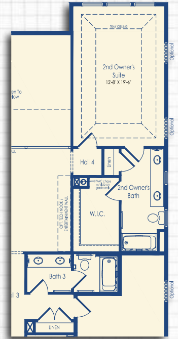
Optional Second Owner's Suite with First Floor 4' Owner's Suite Extension
