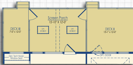
Optional Screen Porch with Optional Decks II & III
