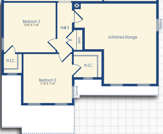
Optional Elevation B Second Floor
