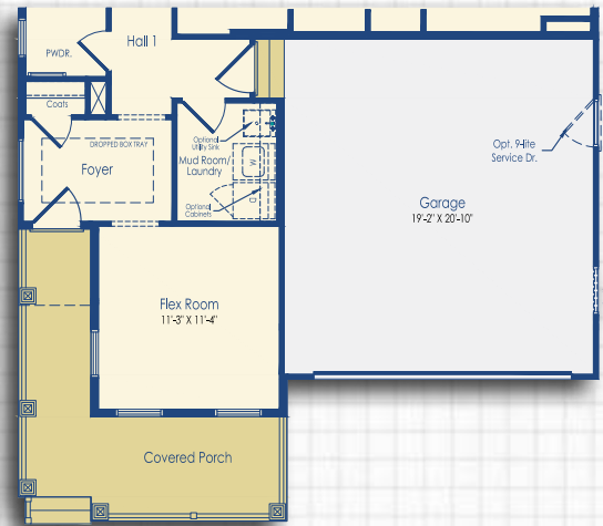
Optional Elevation B First Floor
