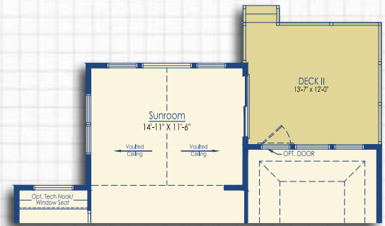
Optional Sunroom and Deck II with 4' Owner's Suite Extension
