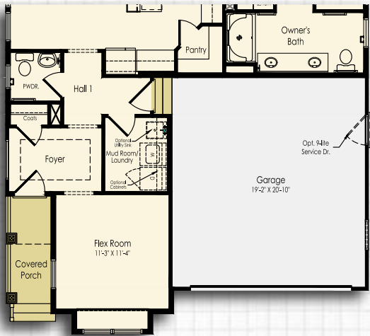
Included Elevation A First Floor
