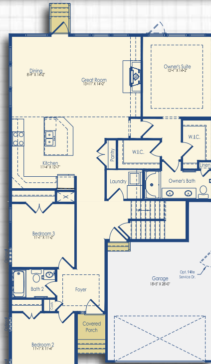
First Floor with Basement/Loft Stairs Schell Style A, B
