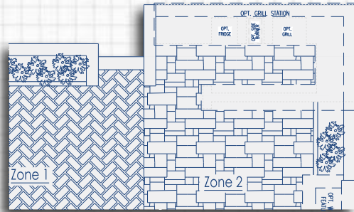
Optional Courtyard with Peninsula Bar
