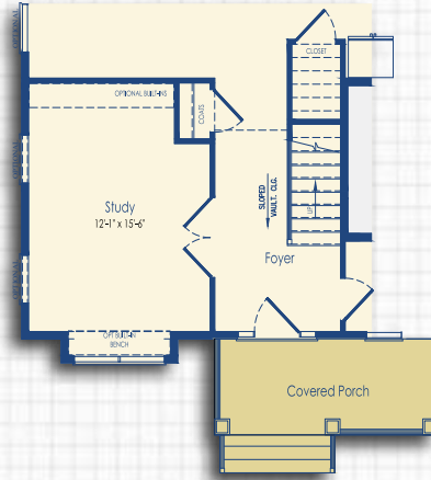
Optional Study *Shown with Elevation A
