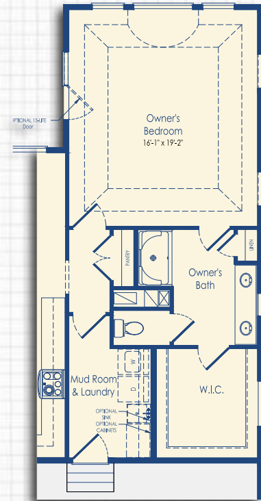
Optional 2' Owner's Suite Ext.
