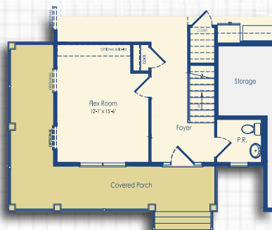
Optional Wrap Around Porch *Elevation C
