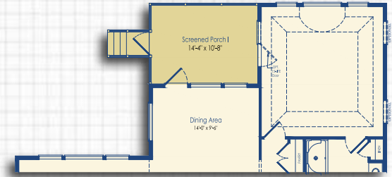
Optional Screened Porch I
