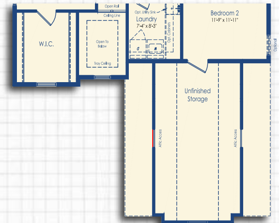
Unfinished Storage with Optional 4ft Garage Extension Ellevation C
