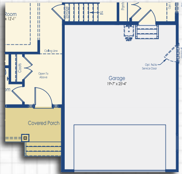
Optional 4' Garage Extension Modern Farmhouse Elevation
