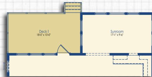
Optional Sunroom with Optional Deck I
