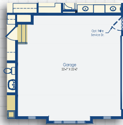
Optional Side Load Craftsman Style
