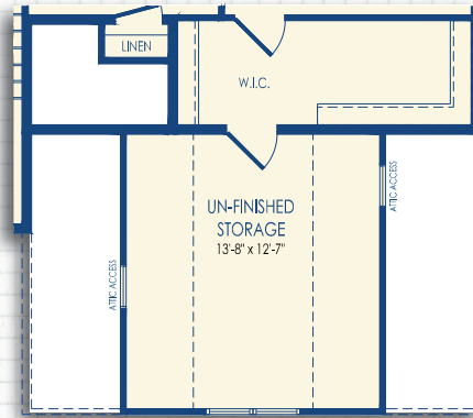
Unfinished Storage with Optional Front Load 4' Garage Extension Second Floor Elevation B
