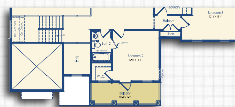
Second Floor Optional Southern Style
