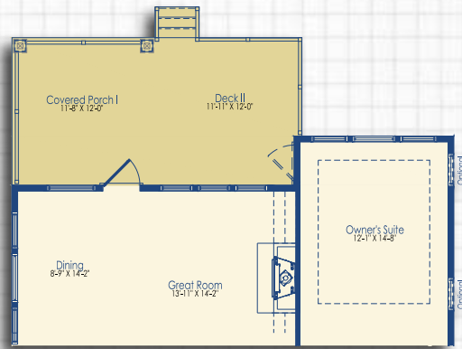
Optional Deck II and Covered Porch I with Luxury Owner's Suite
