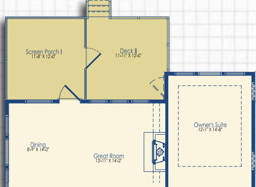
Optional Screen Porch I and Deck III with Luxury Owner's Suite
