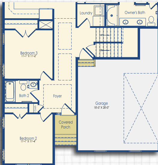
Optional Side Load Garage with Basement/Loft Stairs
