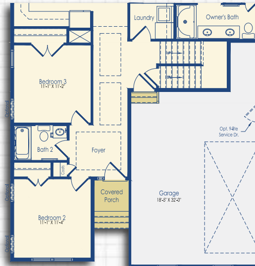
Optional Side Load Garage with 4ft Extension and Basement/Loft Stairs
