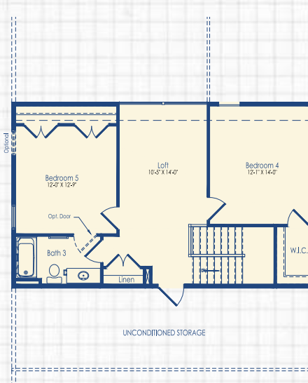
Optional Bedroom 5 and Bath 3 with Bedroom 4 and Loft
