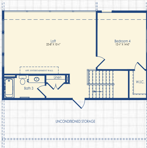
Optional Bedroom 4 and Bath 3 with Loft
