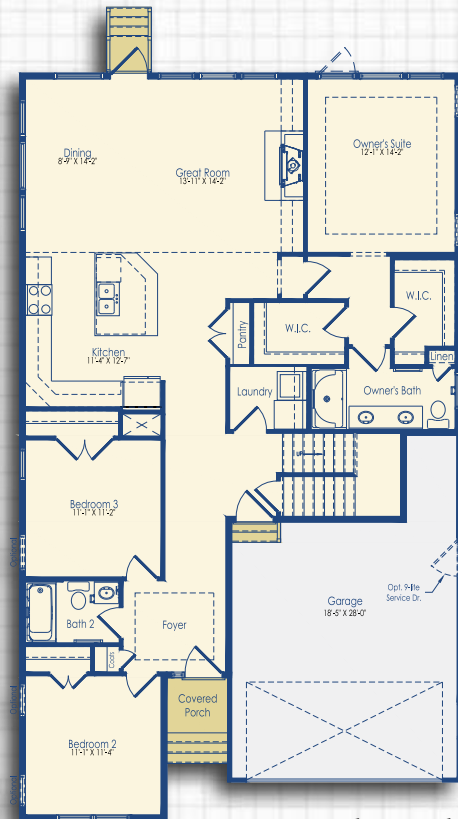
First Floor with Basement/Loft Stairs Schell Style A, B, & Modern Farmhouse
