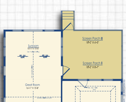
Optional Screen Porch II
