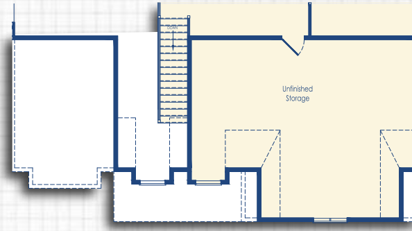
Optional Elevation F Second Floor
