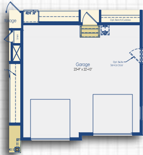
Garage with Optional Second Owner's Suite, Study 2, or Flex Room II Elevation A,
