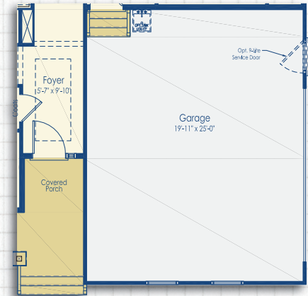
Optional Sideload Garage with 4ft Extension Craftsman Elevation
