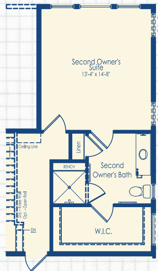
Optional Second Owner's Suite
