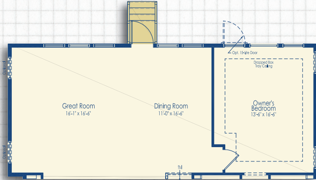
Optional 2ft Great Room and Rear Extension
