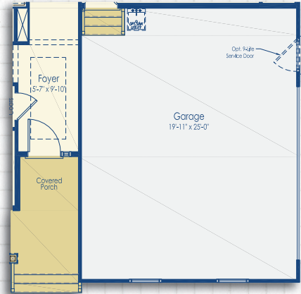
Optional Sideload Garage with 4ft Extension Elevation B
