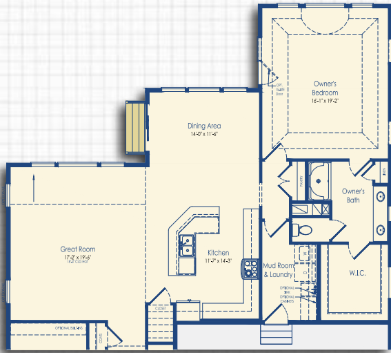
Optional 2' Whole House Rear Extension
