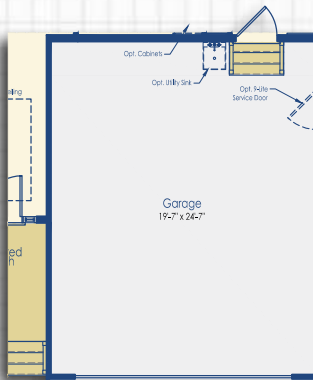
Optional 4' Garage Extension Craftsman Elevation
