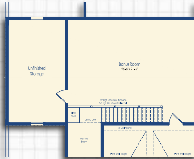
Optional Closed Loft
