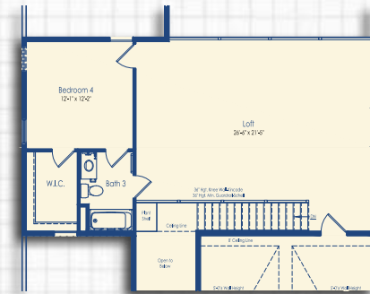
Optional Loft with Bedroom 4 and Bath 3
