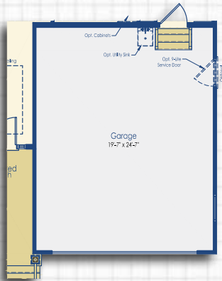
Optional 4' Garage Extension Elevation D
