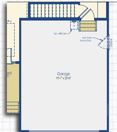
Optional 4' Garage with Basement Stairs Craftsman Elevation
