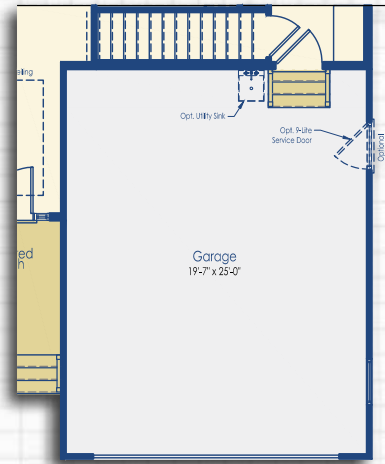
Optional 4' Garage with Basement Stairs Craftsman Elevation
