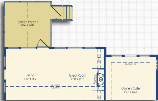
Optional Screen Porch I and Optional Deck II with 2 Ft. Rear Extension
