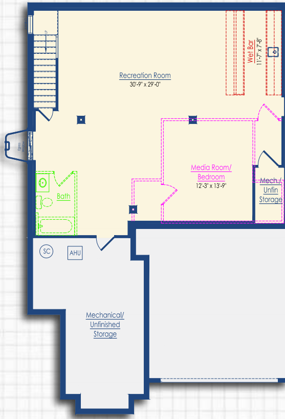
Finished Basement
