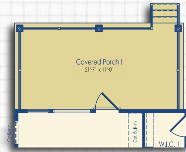
Optional Covered Porch I
