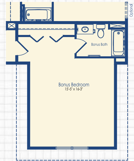
Optional Bonus Bedroom with 4ft Extension Elevation A
