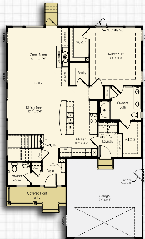
First Floor Elevation A, B, C, Craftsman & Modern Farmhouse
