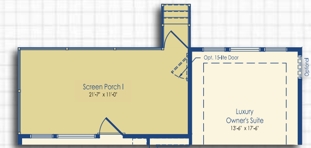
Optional Screen Porch I with Optional Luxury Owner's Suite I/II
