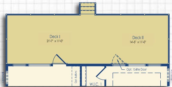
Optional Deck I and II
