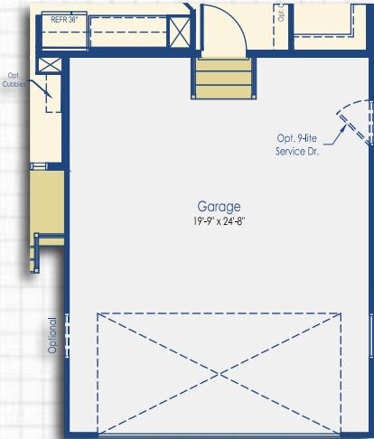
Optional 4ft Garage Extension Elevation A
