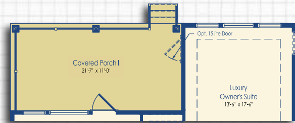
Optional Covered Porch I with Optional Luxury Owner's Suite I/II
