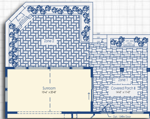
Optional Courtyard with Sunroom and Covered Porch II
