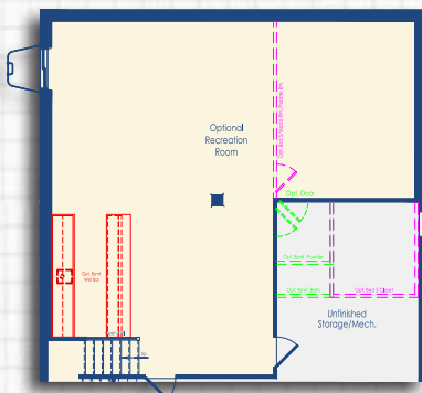
Optional 2Ft Full Rear Extension
