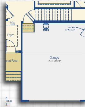
Stairs to Optional Basement
