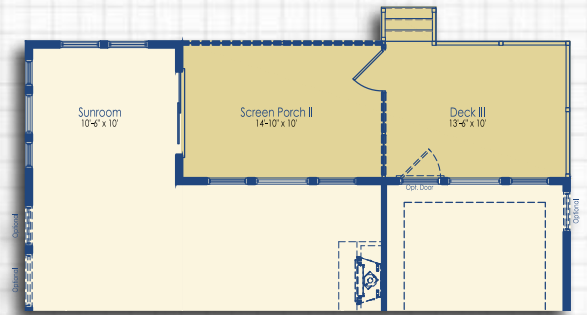
Optional Sunroom with Optional Screen Porch II and Deck III
