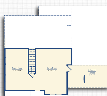
Optional Finished Bonus Room Elevation F
