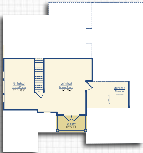
Optional Unfinished Bonus Room Elevation E
