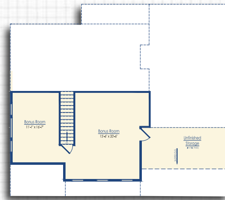
Optional Finished Bonus Room Elevation D *Also available with Open Rail staircase.
