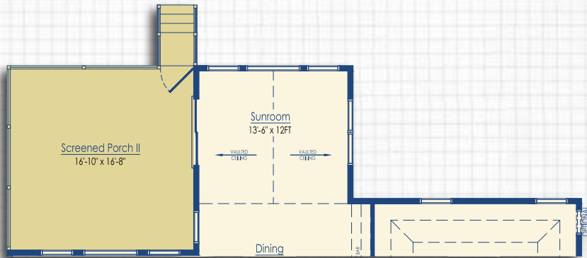
Optional Sunroom with Optional Screened Porch II
