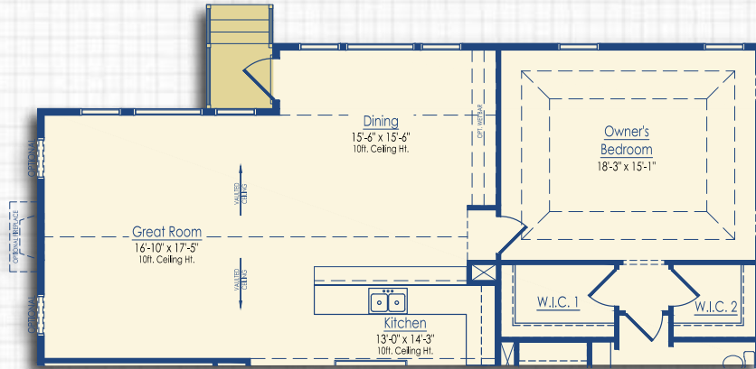
Optional 2' Whole House Rear Extension with Optional Vaulted Ceiling
