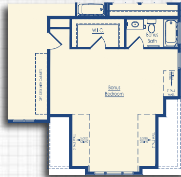
Optional Bonus Bedroom with 4' Garage Extension Craftsman Style
