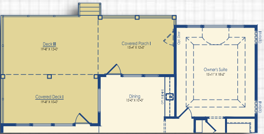
Optional Covered Porch I with Covered Deck I with Decks III and IV
