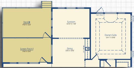
Optional Sunroom I and Screen Porch I with Decks III and IV Above
