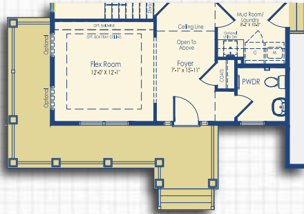
Optional Wrap Around Porch Included Schell Style B
