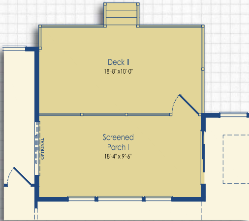
Optional Screened Porch I with Optional Deck II
