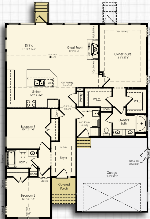
Included Schell Style A First Floor
