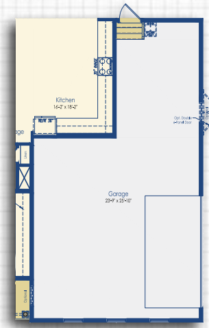
Optional Sideload Garage Southern Farmhouse
