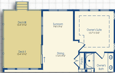
Optional Sunroom with Optional Deck I and Optional Deck III
