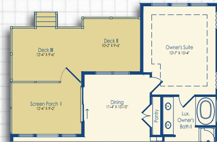
Optional Screen Porch I, Optional Deck II and Optional Deck III with Optional Luxury Owner's Suite I or II
