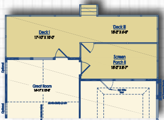
Optional Screen Porch II with Decks I and III with Luxury Owner's Suite I or II
