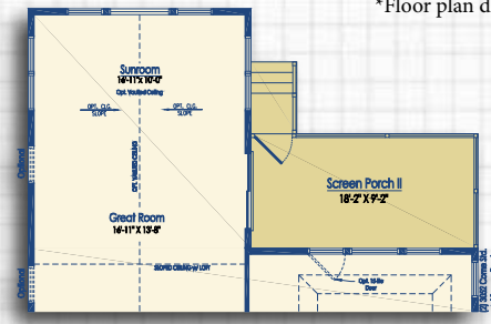
Optional Sunroom with Screen Porch II
