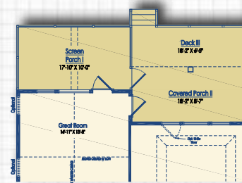
Optional Screen Porch I and Deck III and Covered Porch II with Luxury Owner's Suite I or II
