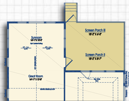
Optional Sunroom with Screen Porch II and III
