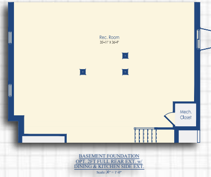
Basement Foundation with Optional 2Ft Full Rear Extension and Dining & Kitchen Side Extension
