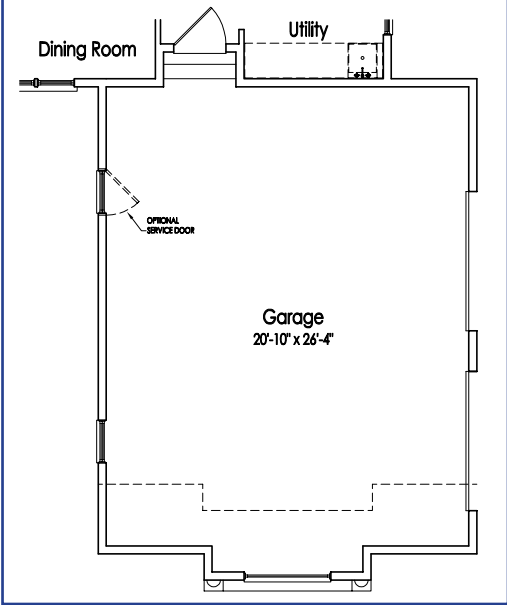
OPTIONAL SIDE LOAD GARAGE W/ 4' EXT.
