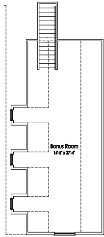
UNFINISHED / FINISHED BONUS ROOM W/ BASEMENT
