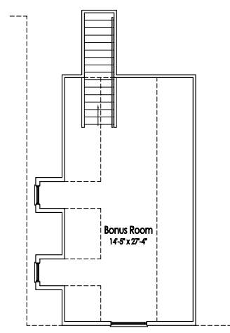
UNFINISHED / FINISHED BONUS ROOM W/ BASEMENT
