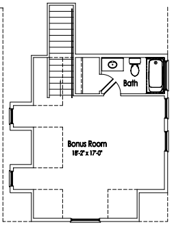
FINISHED BONUS ROOM W/ BATH & CRAWL
