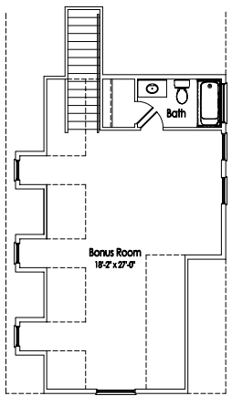
FINISHED BONUS ROOM W/ BATH & CRAWL
