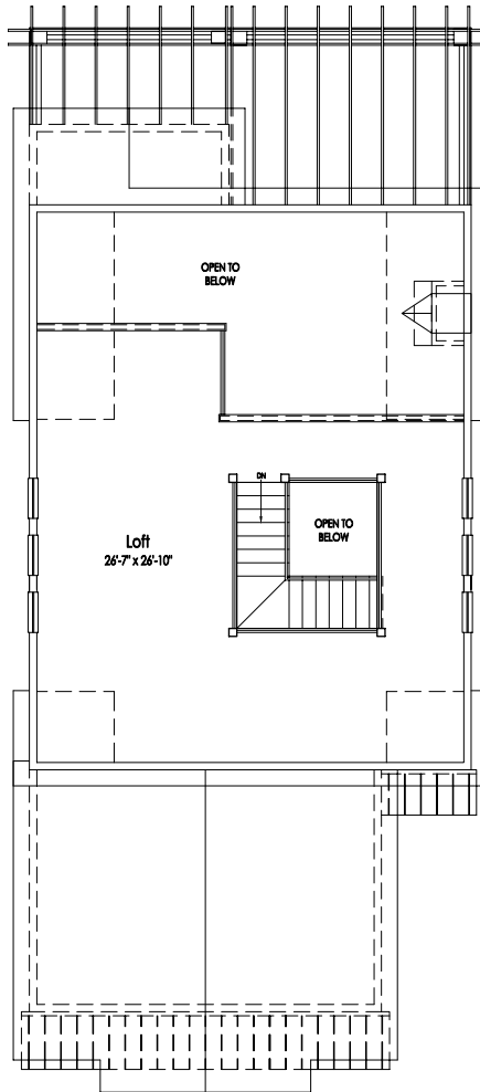
Optional Third Floor Loft Plan
