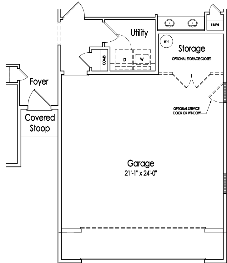
Optional 4' Garage Extension (Shown with Optional Storage Closet)
