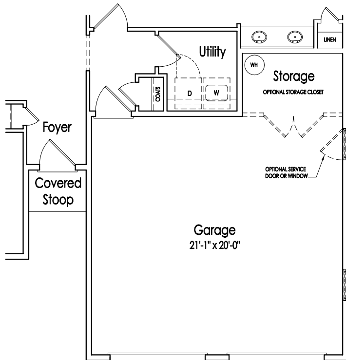
Optional 2-Door Garage (Shown with Optional Storage Closet)
