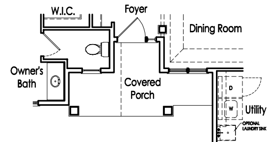
Covered Porch with Elevation B
