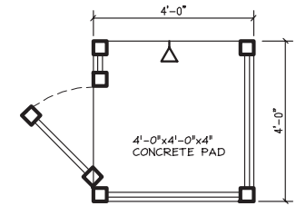
4' X 4' OUTDOOR SHOWER
