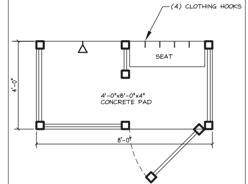
4' X 8' OUTDOOR SHOWER
