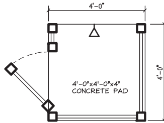
4' X 4' OUTDOOR SHOWER
