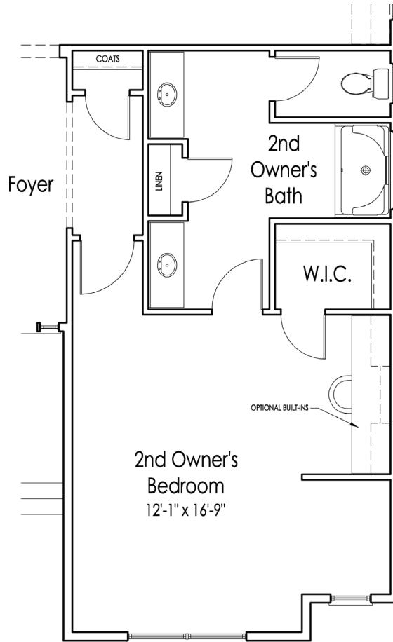
OPTIONAL 2ND OWNER'S BEDROOM - ELEVATION B
