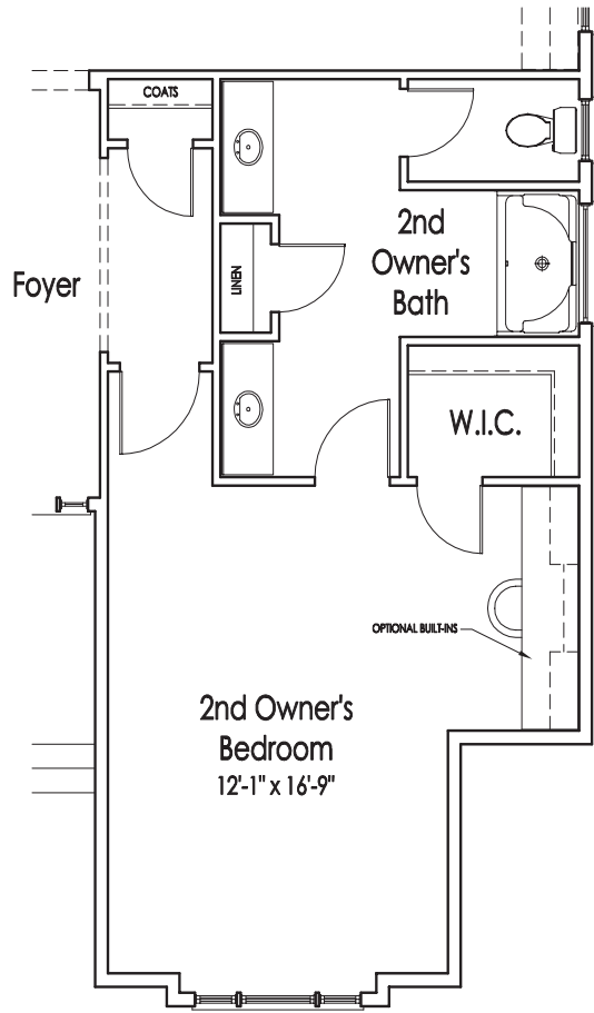
OPTIONAL 2ND OWNER'S BEDROOM - ELEVATION A
